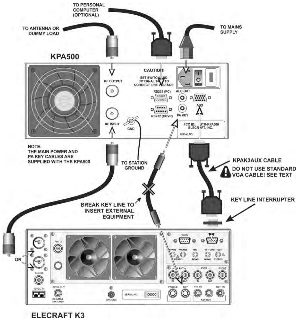
Figure 4. K3 Enhanced Cabling Using KPAK3AUX Cable and Separate Key Line.
